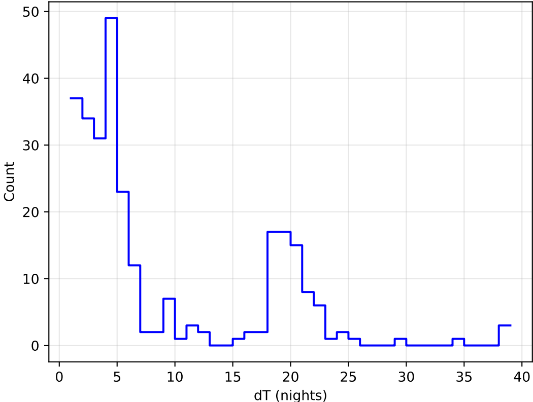
ddf_acor_sf10_Isf40_Isr20_v3.4_10yrs all bands: DD:EDFS Delta Nights Histogram
