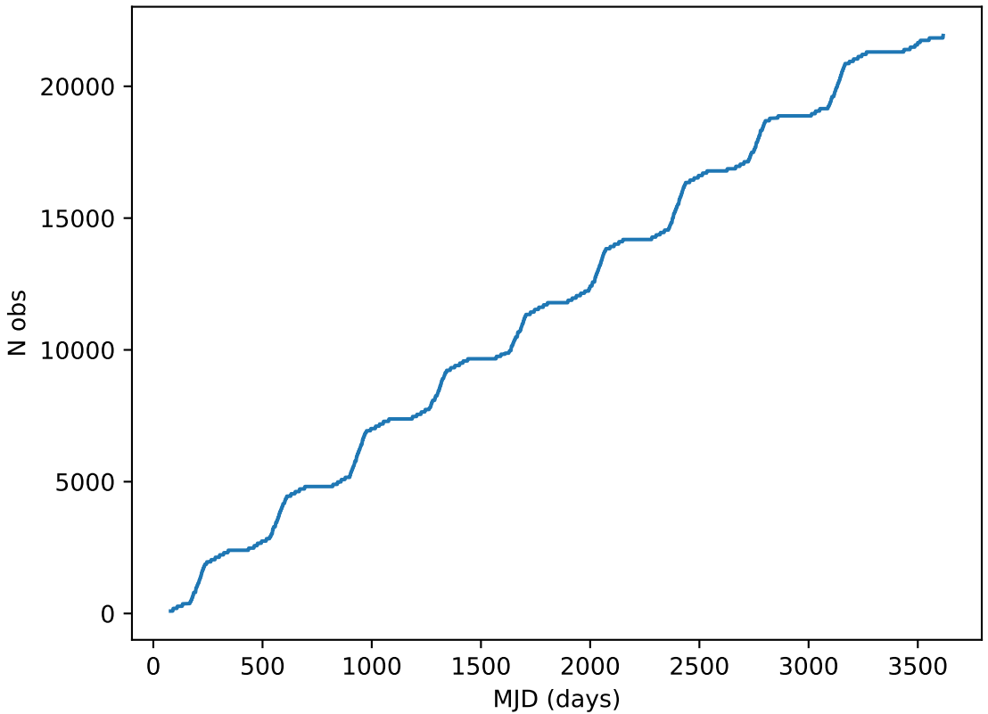
ddf_acor_sf10_lsf40_lsr20_v3.4_10yrs all bands: DD:EDFS Cumulative NVisits
