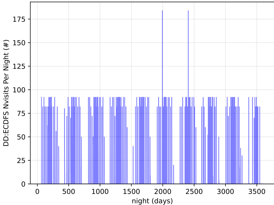
ddf_acor_sf10_lsf40_lsr20_v3.4_10yrs all bands: DD:ECDFS Nvisits Per Night
