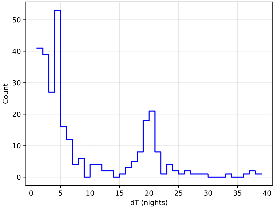
ddf_acor_sf10_lsf40_lsr20_v3.4_10yrs all bands: DD:ECDFS Delta Nights Histogram
