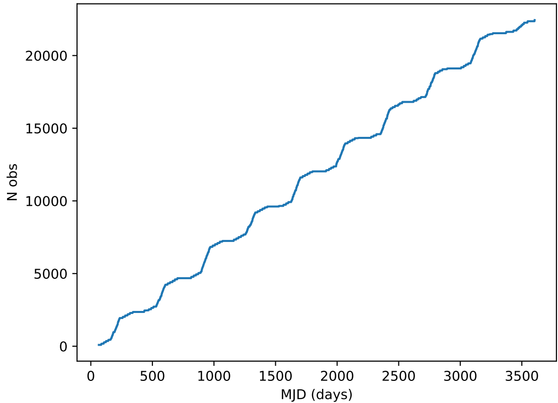
ddf_acor_sf10_lsf40_lsr20_v3.4_10yrs all bands: DD:ECDFS Cumulative NVisits
