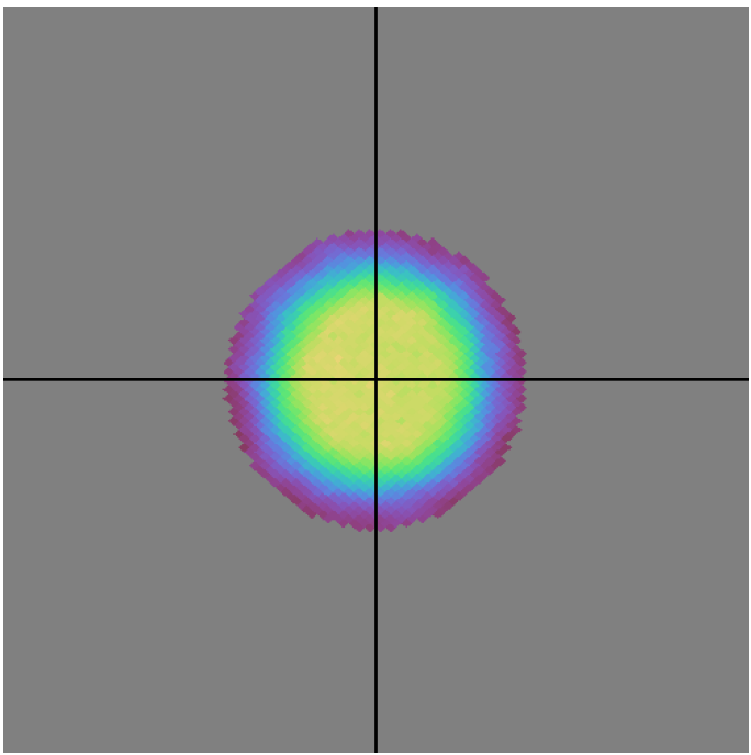
ddf_acor_sf10_lsf40_lsr20_v3.4_10yrs all bands: DD:COSMOS N Unique Nights
