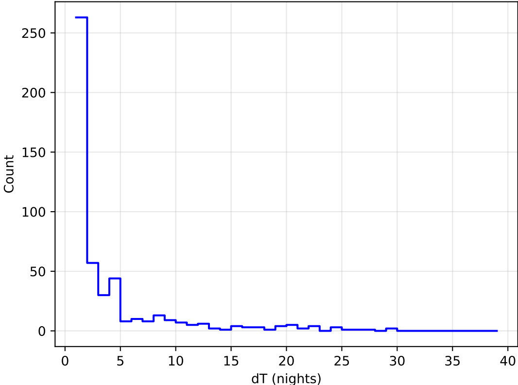
ddf_acor_sf10_Isf40_Isr20_v3.4_10yrs all bands: DD:COSMOS Delta Nights Histogram
