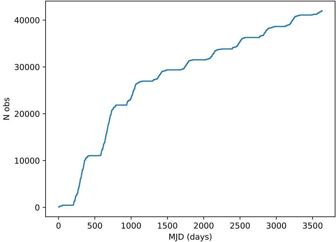
ddf_acor_sf10_lsf40_lsr20_v3.4_10yrs all bands: DD: COSMOS Cumulative NVisits
