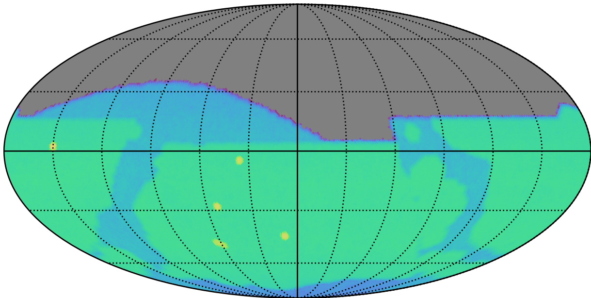
ddf_acor_sf10_lsf40_lsr10_v3.4_10yrs i: SurfaceBrightLimit
