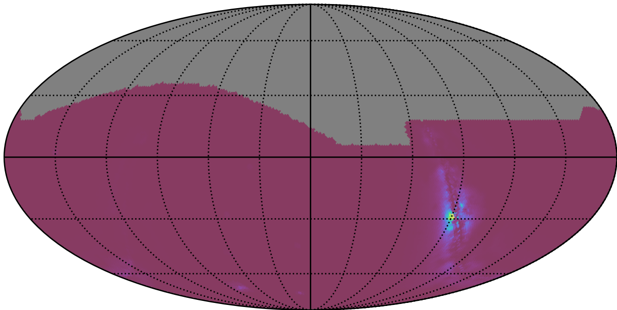
ddf_acor_sf10_lsf40_lsr10_v3.4_10yrs : NlcPoints
