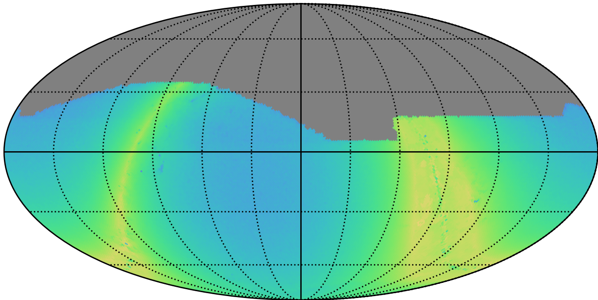
ddf_acor_sf10_lsf40_lsr10_v3.4_10yrs i: N stars to Precision 0.20
