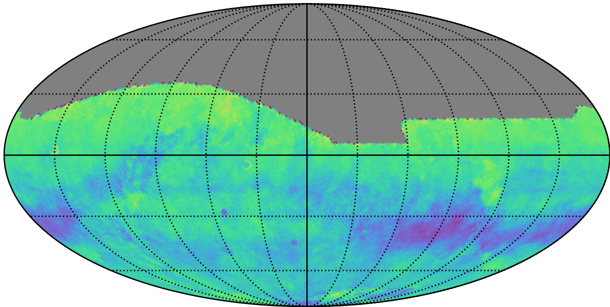
ddf_acor_sf10_lsf40_lsr10_v3.4_10yrs r: Kuiper rotSkyPos
