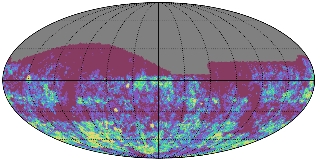
ddf_acor_sf10_lsf40_lsr10_v3.4_10yrs r band: Gaps_3hr
