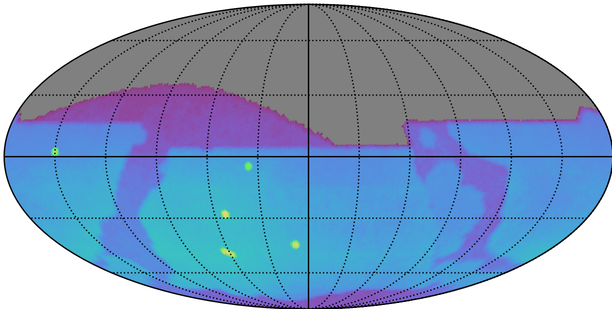
ddf_acor_sf10_lsf40_lsr10_v3.4_10yrs : Brown Dwarf, L7
