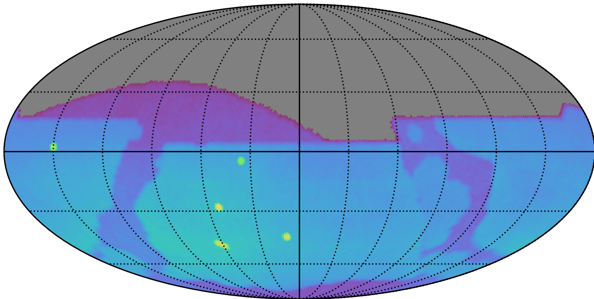
ddf_acor_sf10_lsf40_lsr10_v3.4_10yrs : Brown Dwarf, L4
