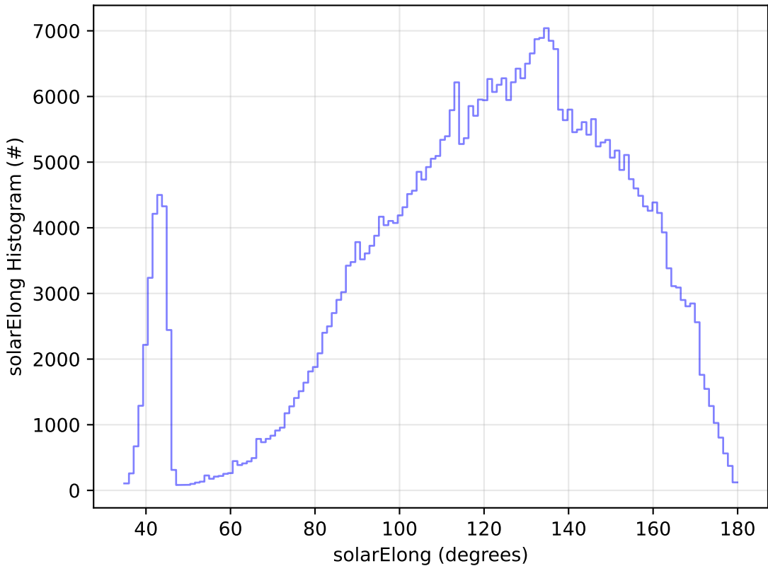
ddf_acor_sf10_lsf40_lsr10_v3.4_10yrs WFD z band: solarElong Histogram
