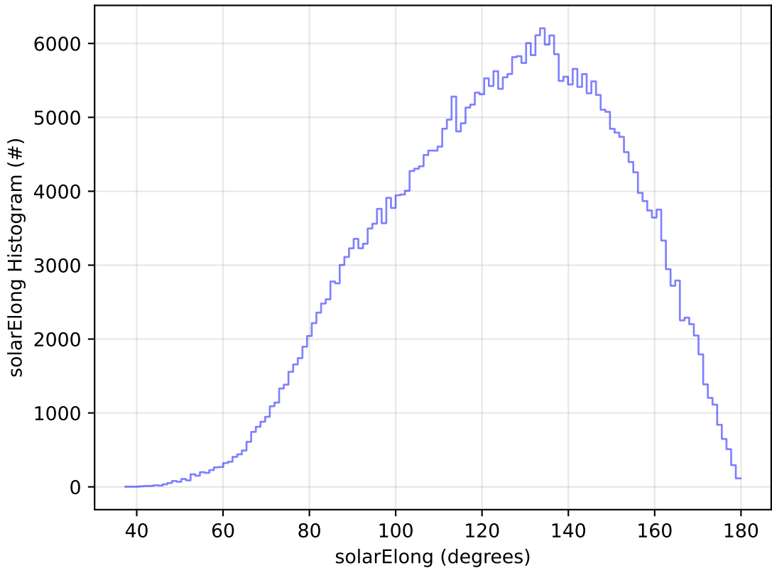
ddf_acor_sf10_lsf40_lsr10_v3.4_10yrs WFD y band: solarElong Histogram
