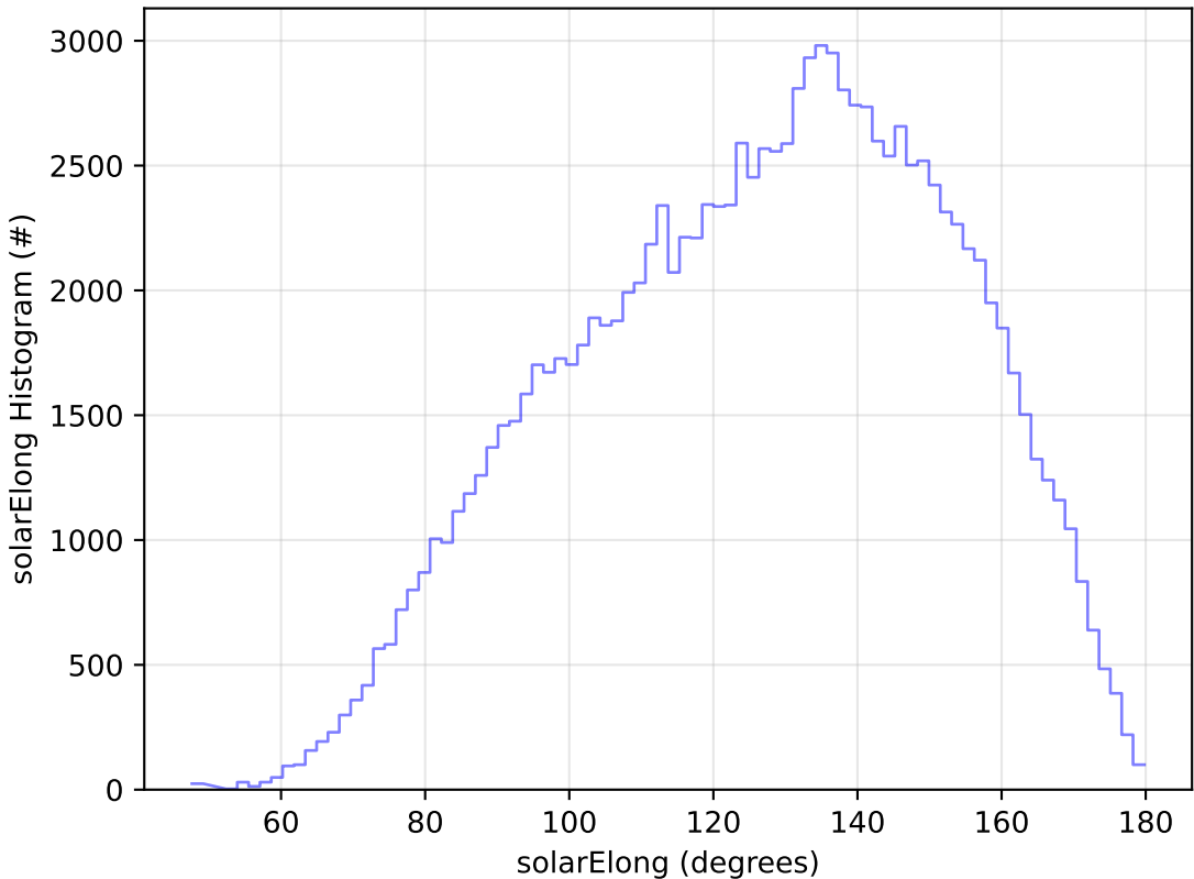
ddf_acor_sf10_lsf40_lsr10_v3.4_10yrs WFD u band: solarElong Histogram
