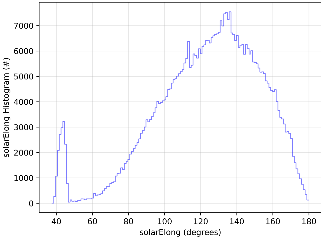
ddf_acor_sf10_lsf40_lsr10_v3.4_10yrs WFD r band: solarElong Histogram
