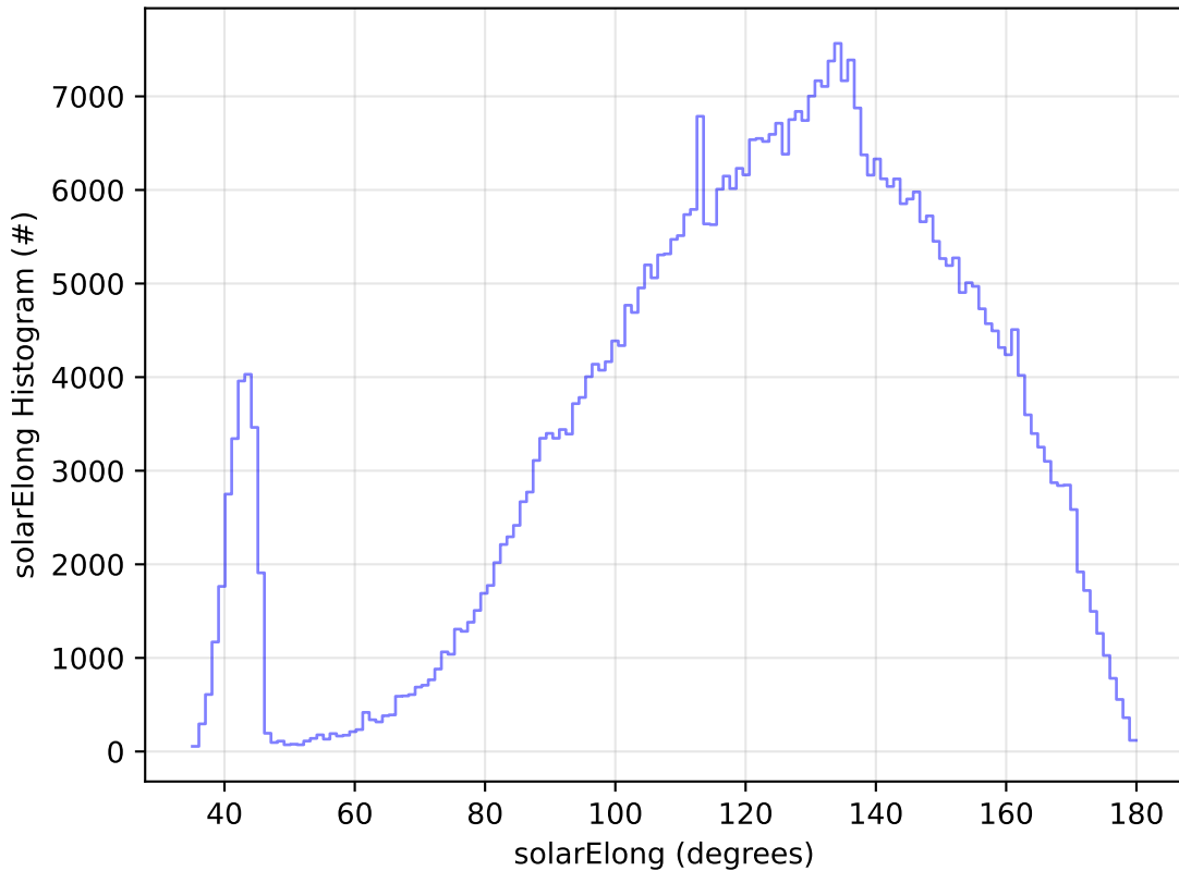
ddf_acor_sf10_lsf40_lsr10_v3.4_10yrs WFD i band: solarElong Histogram
