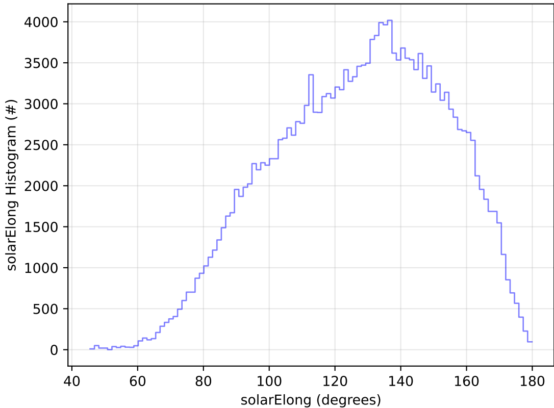
ddf_acor_sf10_ls40_lsr10_v3.4_10yrs WFD g band: solarElong Histogram
