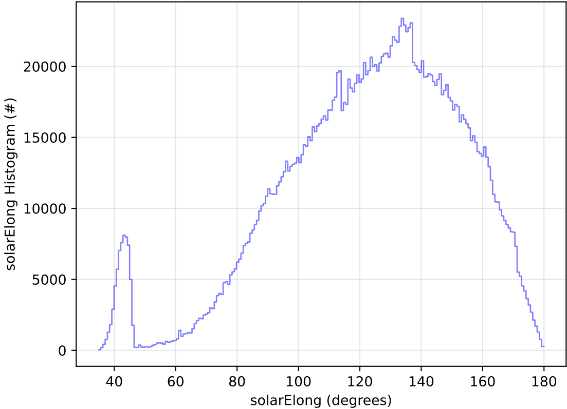
ddf_acor_sf10_lsf40_lsr10_v3.4_10yrs WFD all bands: solarElong Histogram
