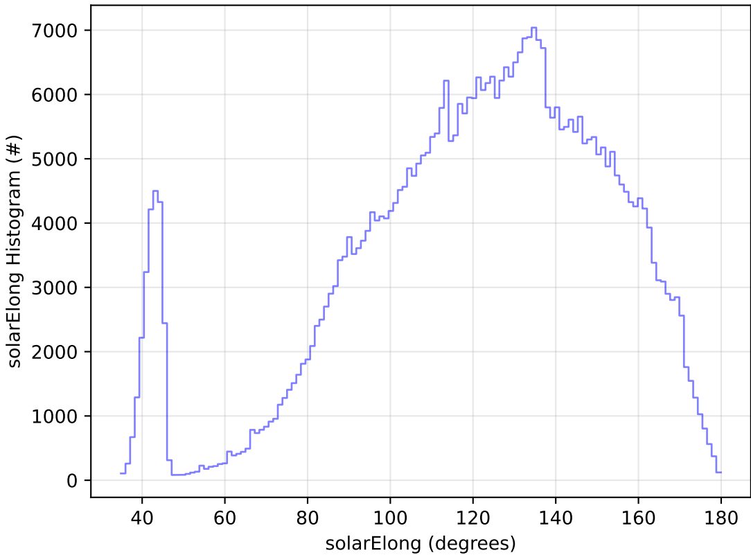
ddf_acor_sf10_lsf40_lsr10_v3.4_10yrs All sky z band: solarElong Histogram
