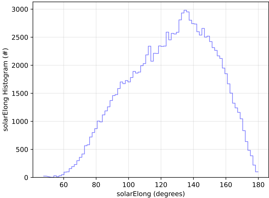
ddf_acor_sf10_lsf40_lsr10_v3.4_10yrs All sky u band: solarElong Histogram
