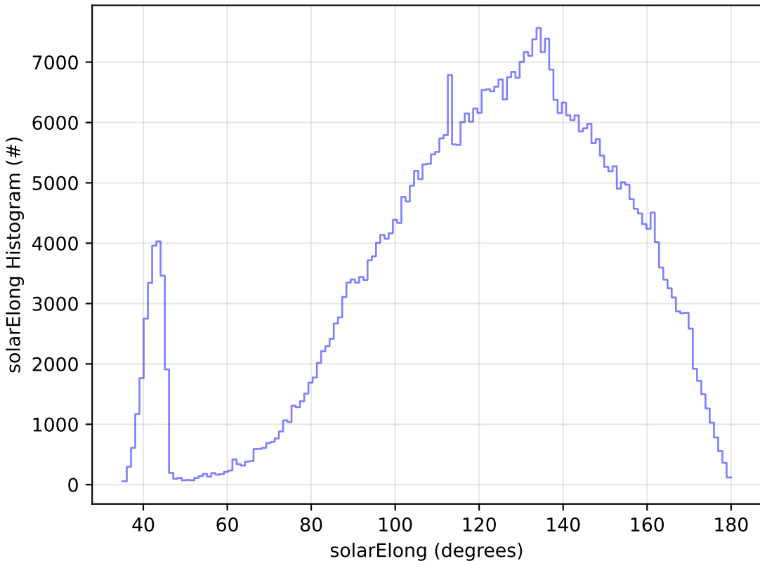
ddf_acor_sf10_lsf40_lsr10_v3.4_10yrs All sky i band: solarElong Histogram
