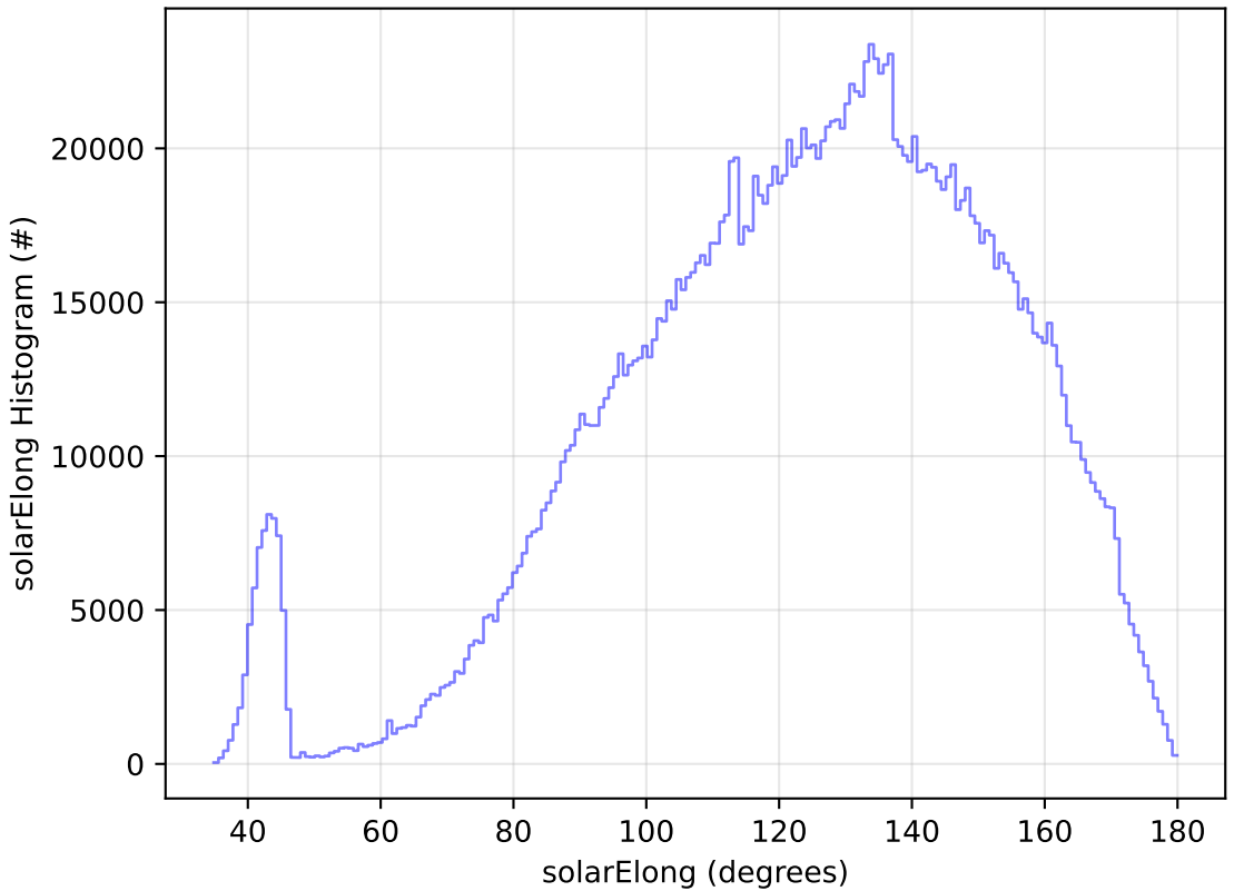
ddf_acor_sf10_lsf40_lsr10_v3.4_10yrs All sky all bands: solarElong Histogram
