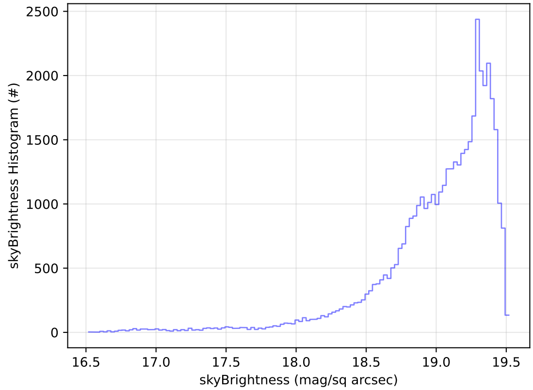
ddf_acor_sf10_lsf40_lsr10_v3.4_10yrs Yr 1 z band: skyBrightness Histogram
