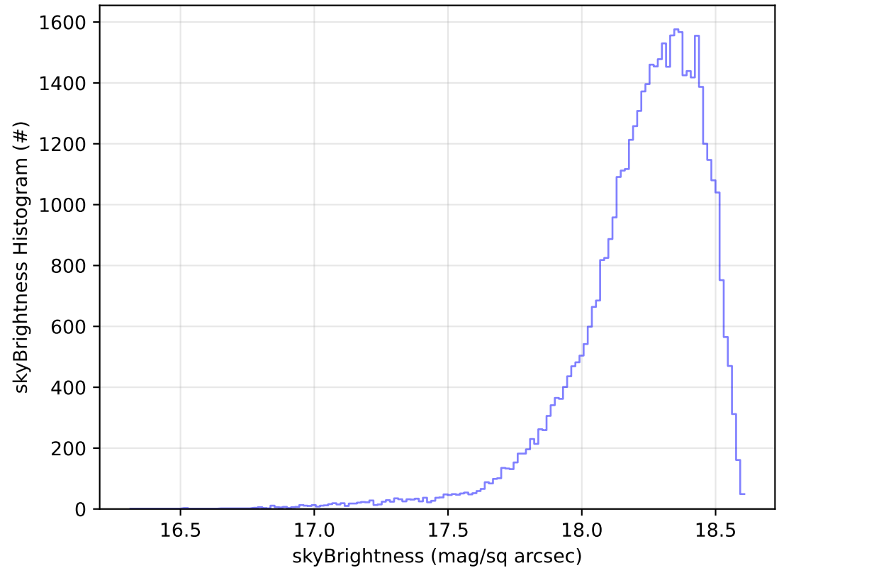
ddf_acor_sf10_lsf40_lsr10_v3.4_10yrs Yr 1 y band: skyBrightness Histogram
