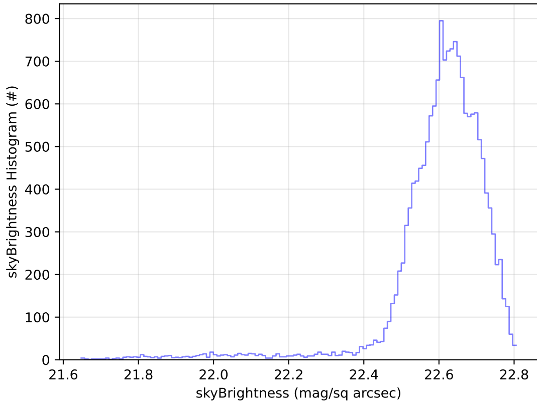
ddf_acor_sf10_lsf40_lsr10_v3.4_10yrs Yr 1 u band: skyBrightness Histogram
