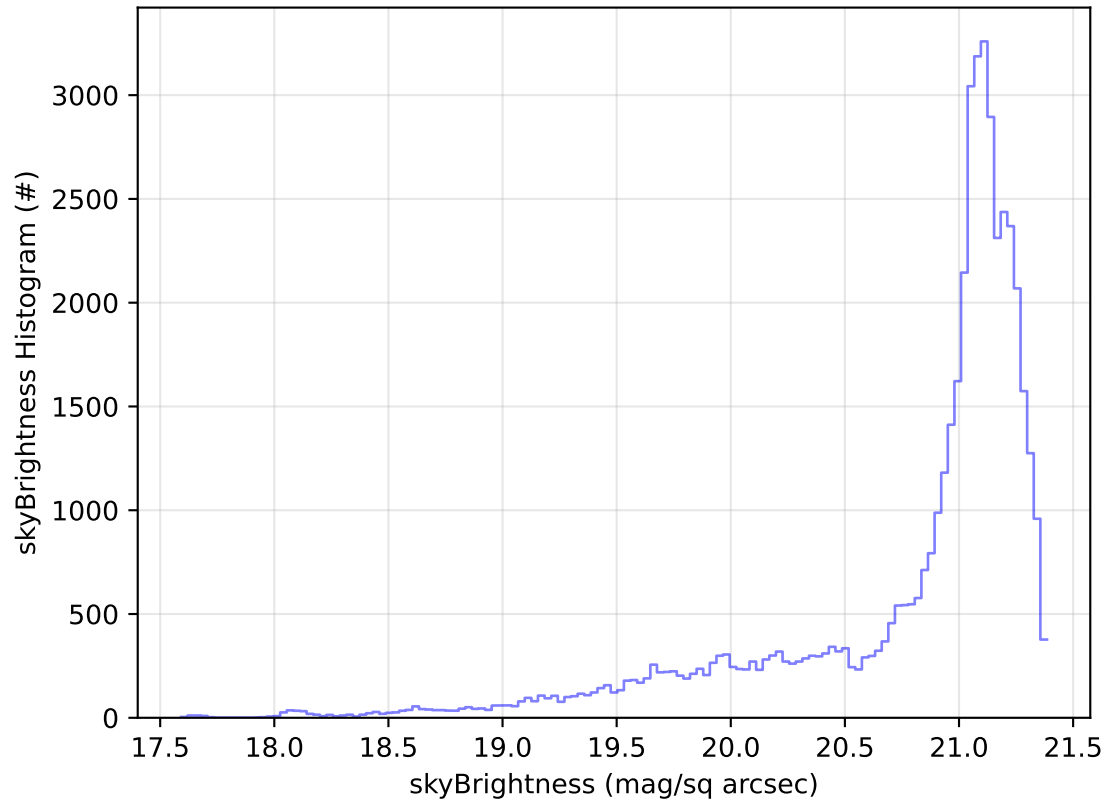
ddf_acor_sf10_lsf40_lsr10_v3.4_10yrs Yr 1 r band: skyBrightness Histogram
