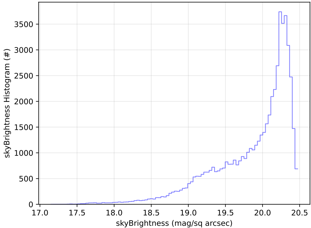
ddf_acor_sf10_lsf40_lsr10_v3.4_10yrs Yr 1 i band: skyBrightness Histogram
