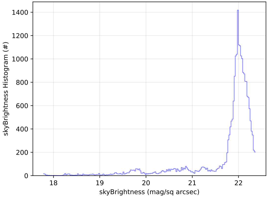
ddf_acor_sf10_lsf40_lsr10_v3.4_10yrs Yr 1 g band: skyBrightness Histogram
