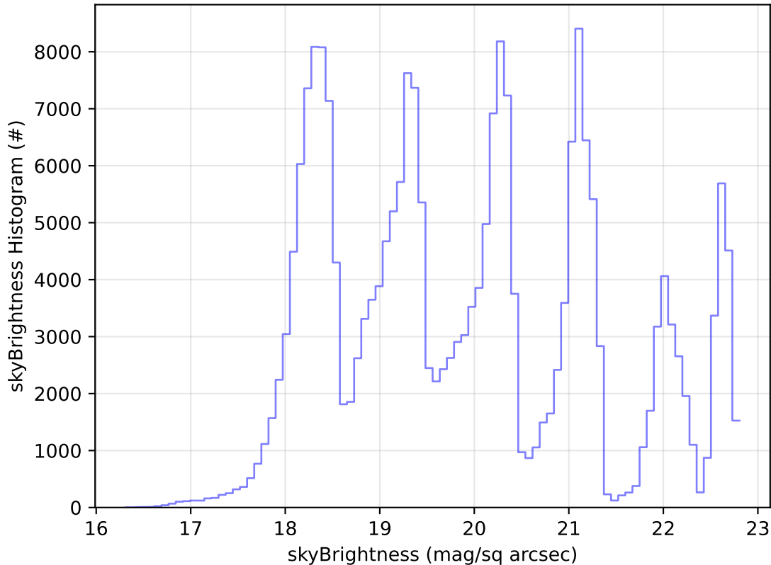
ddf_acor_sf10_lsf40_lsr10_v3.4_10yrs Yr 1 all bands: skyBrightness Histogram
