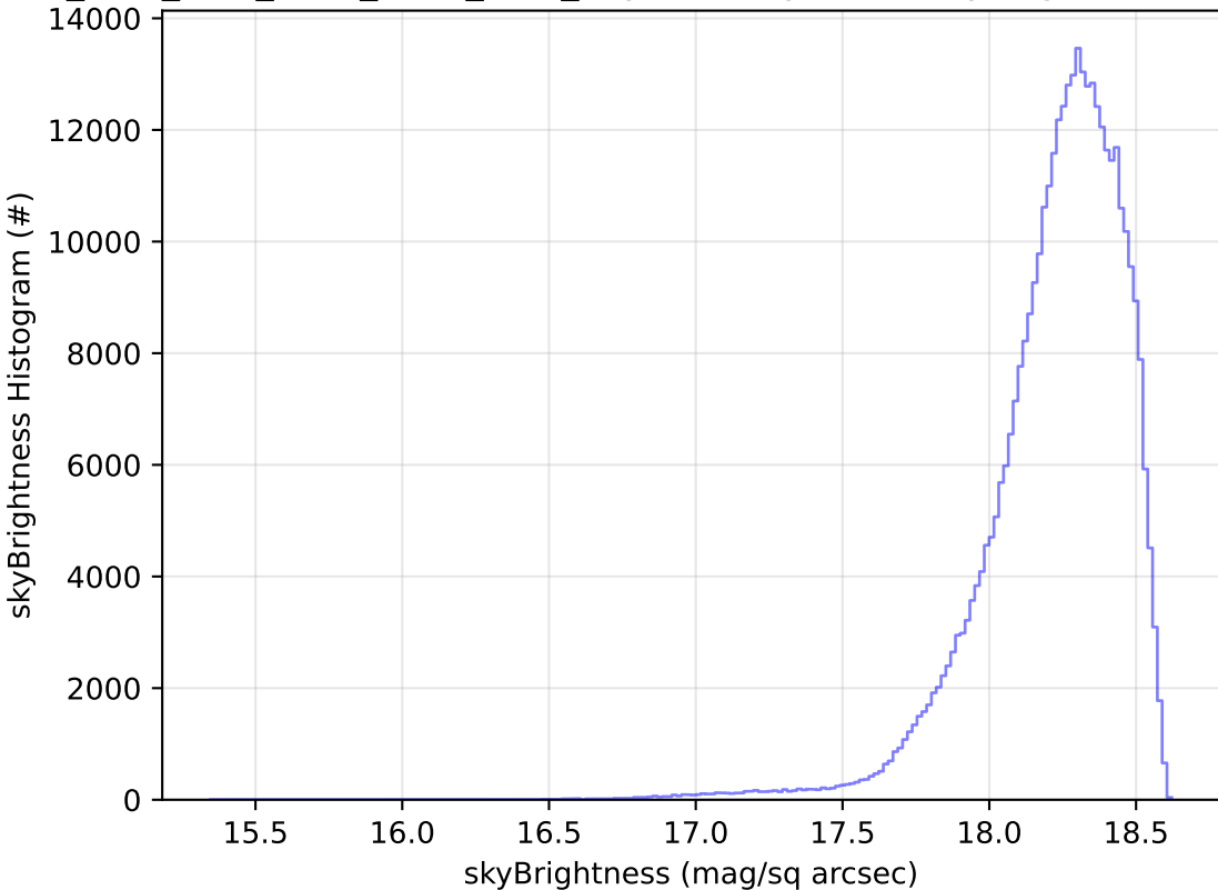
ddf_acor_sf10_lsf40_lsr10_v3.4_10yrs WFD y band: skyBrightness Histogram
