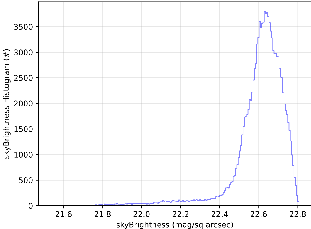
ddf_acor_sf10_lsf40_lsr10_v3.4_10yrs WFD u band: skyBrightness Histogram
