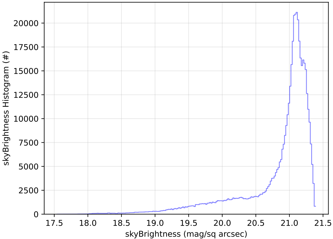
ddf_acor_sf10_lsf40_lsr10_v3.4_10yrs WFD r band: skyBrightness Histogram
