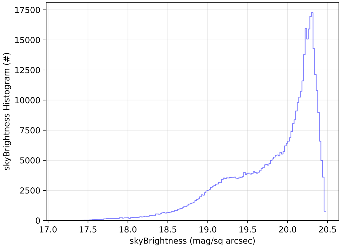
ddf_acor_sf10_lsf40_lsr10_v3.4_10yrs WFD i band: skyBrightness Histogram
