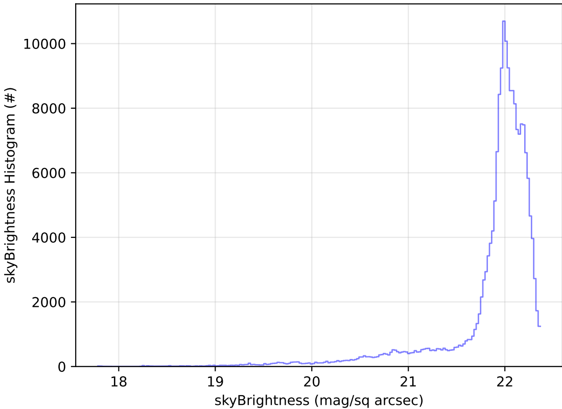
ddf_acor_sf10_lsf40_lsr10_v3.4_10yrs WFD g band: skyBrightness Histogram
