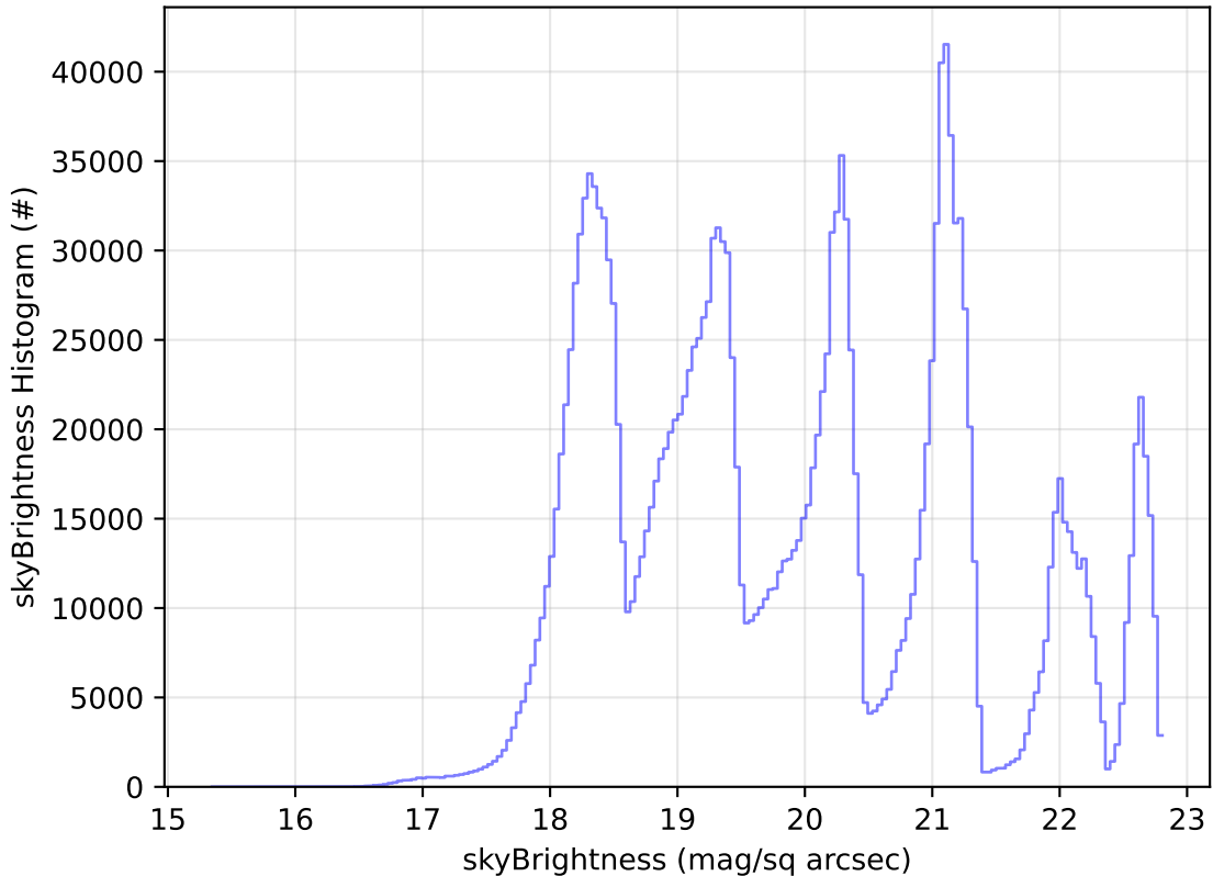
ddf_acor_sf10_ls40_lsr10_v3.4_10yrs WFD all bands: skyBrightness Histogram
