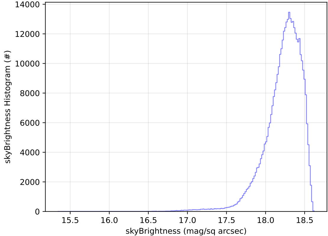
ddf_acor_sf10_lsf40_lsr10_v3.4_10yrs All sky y band: skyBrightness Histogram
