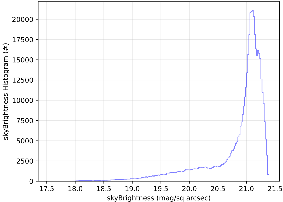
ddf_acor_sf10_lsf40_lsr10_v3.4_10yrs All sky r band: skyBrightness Histogram
