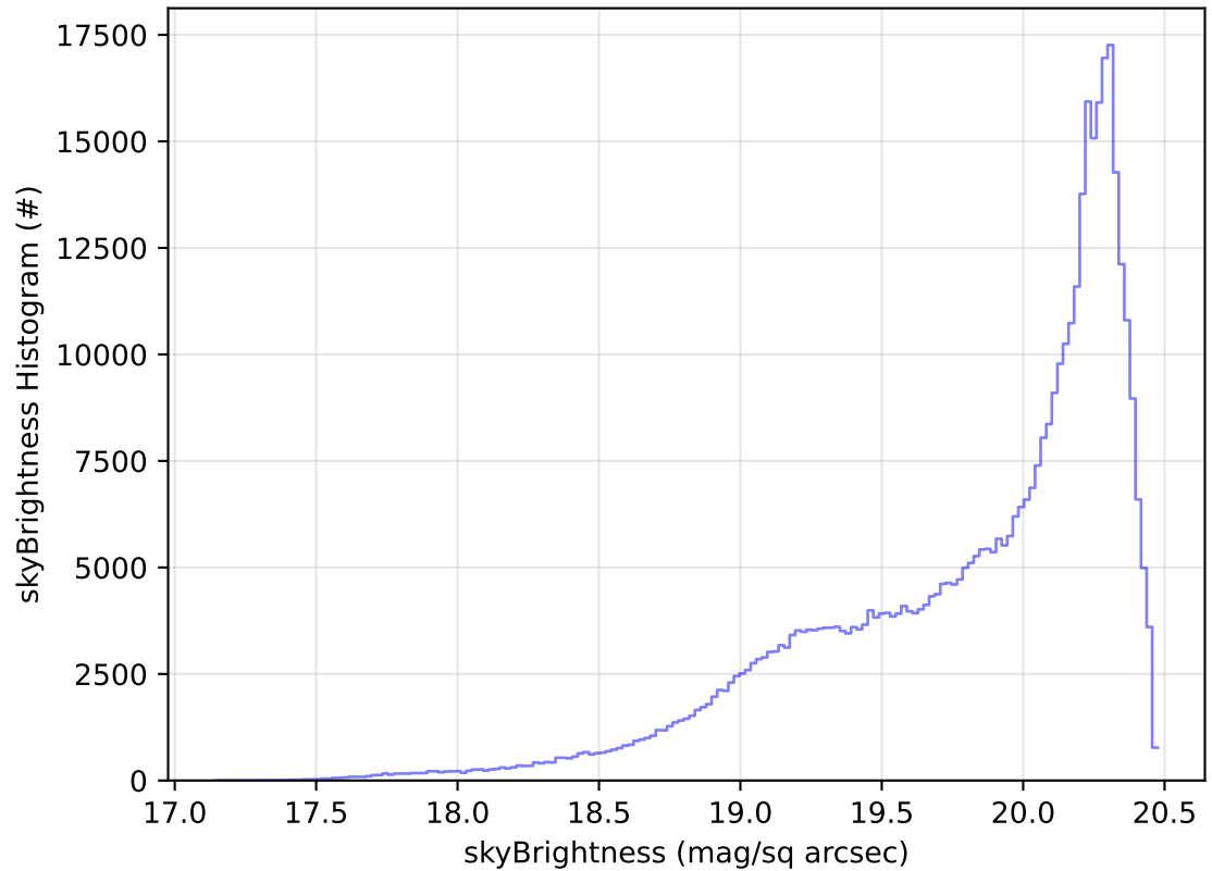
ddf_acor_sf10_lsf40_lsr10_v3.4_10yrs All sky i band: skyBrightness Histogram
