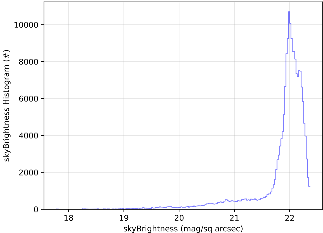
ddf_acor_sf10_lsf40_lsr10_v3.4_10yrs All sky g band: skyBrightness Histogram
