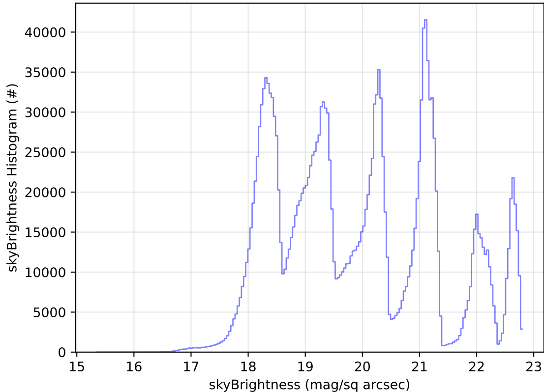
ddf_acor_sf10_lsf40_lsr10_v3.4_10yrs All sky all bands: skyBrightness Histogram
