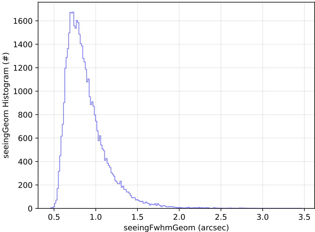
ddf_acor_sf10_lsf40_lsr10_v3.4_10yrs Yr 1 z band: seeingGeom Histogram
