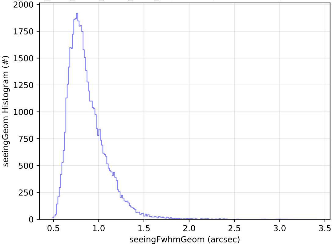
ddf_acor_sf10_lsf40_lsr10_v3.4_10yrs Yr 1 y band: seeingGeom Histogram
