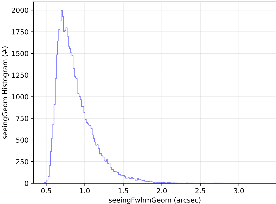
ddf_acor_sf10_lsf40_lsr10_v3.4_10yrs Yr 1 r band: seeingGeom Histogram
