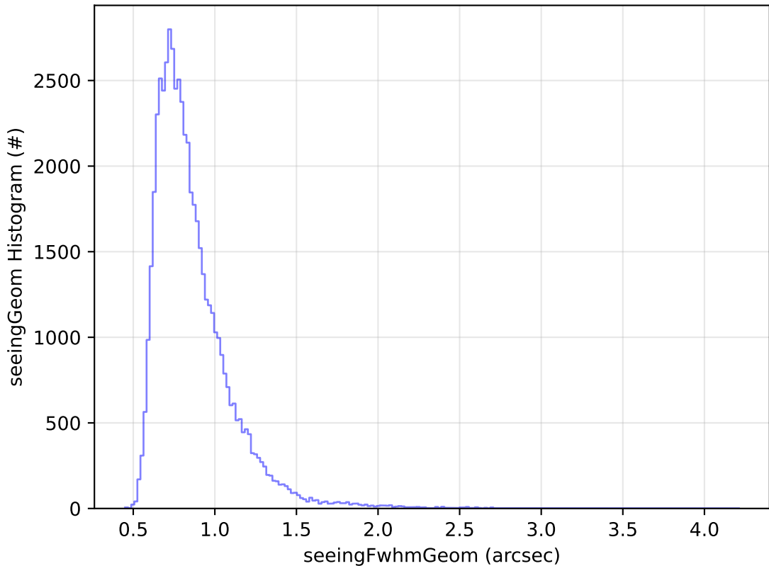
ddf_acor_sf10_lsf40_lsr10_v3.4_10yrs Yr 1 i band: seeingGeom Histogram
