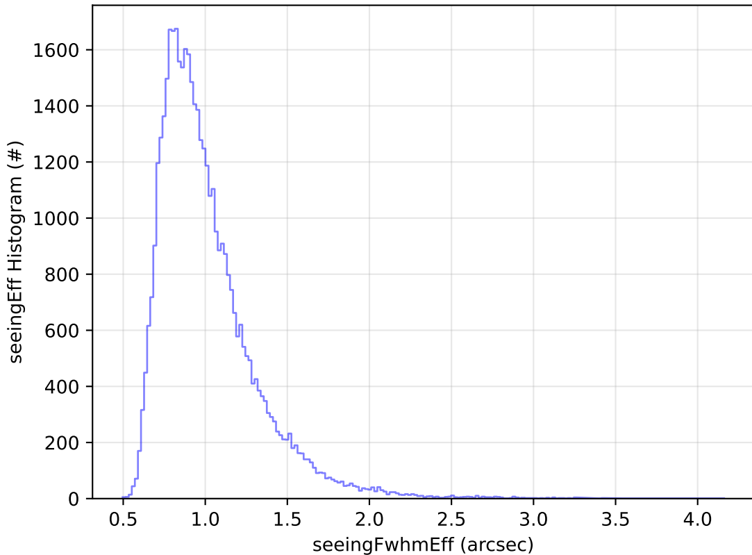
ddf_acor_sf10_lsf40_lsr10_v3.4_10yrs Yr 1 z band: seeingEff Histogram
