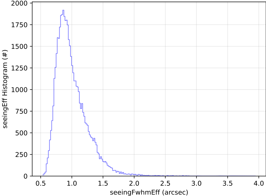
ddf_acor_sf10_lsf40_lsr10_v3.4_10yrs Yr 1 y band: seeingEff Histogram
